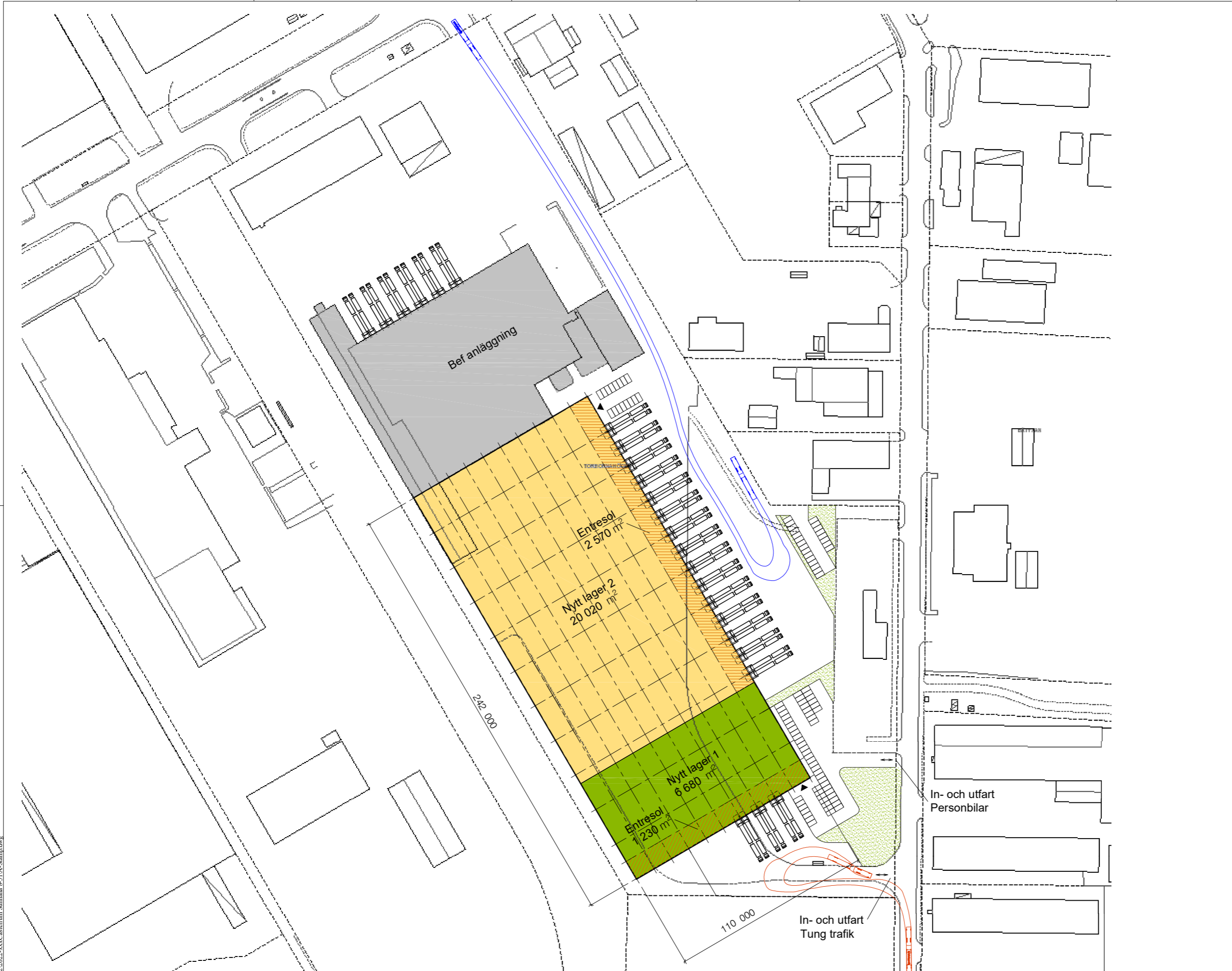
Situationsplan - ALT 3 1:1000
