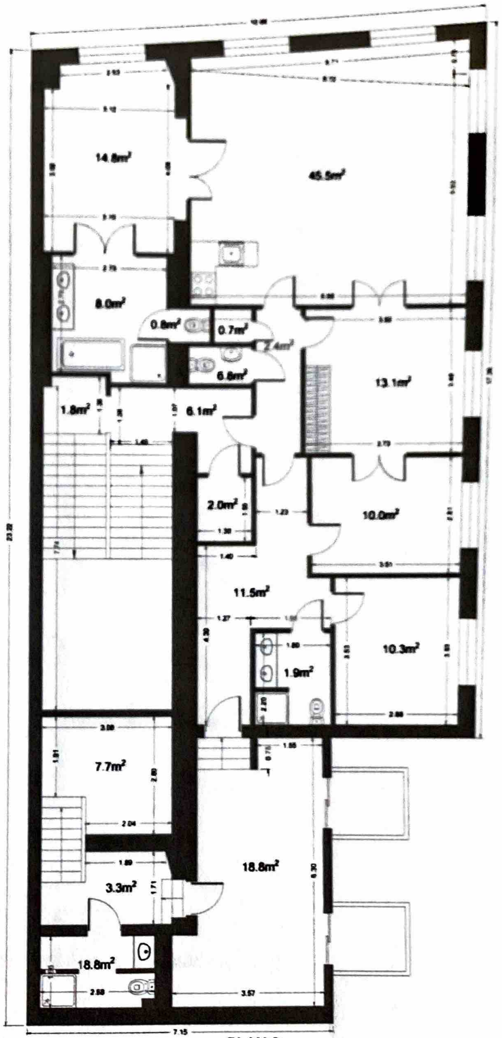
PLAN 3
