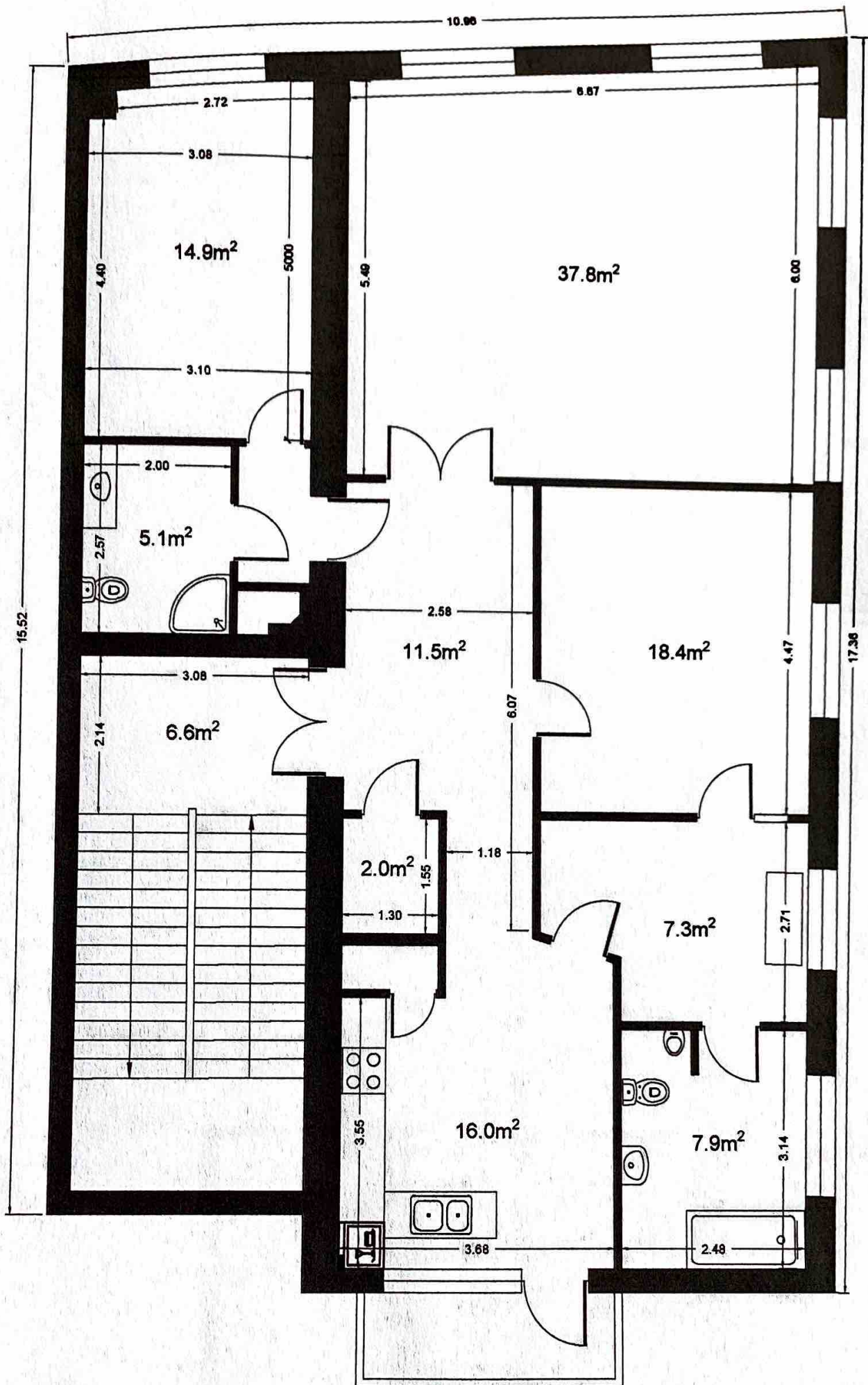
PLAN 4
