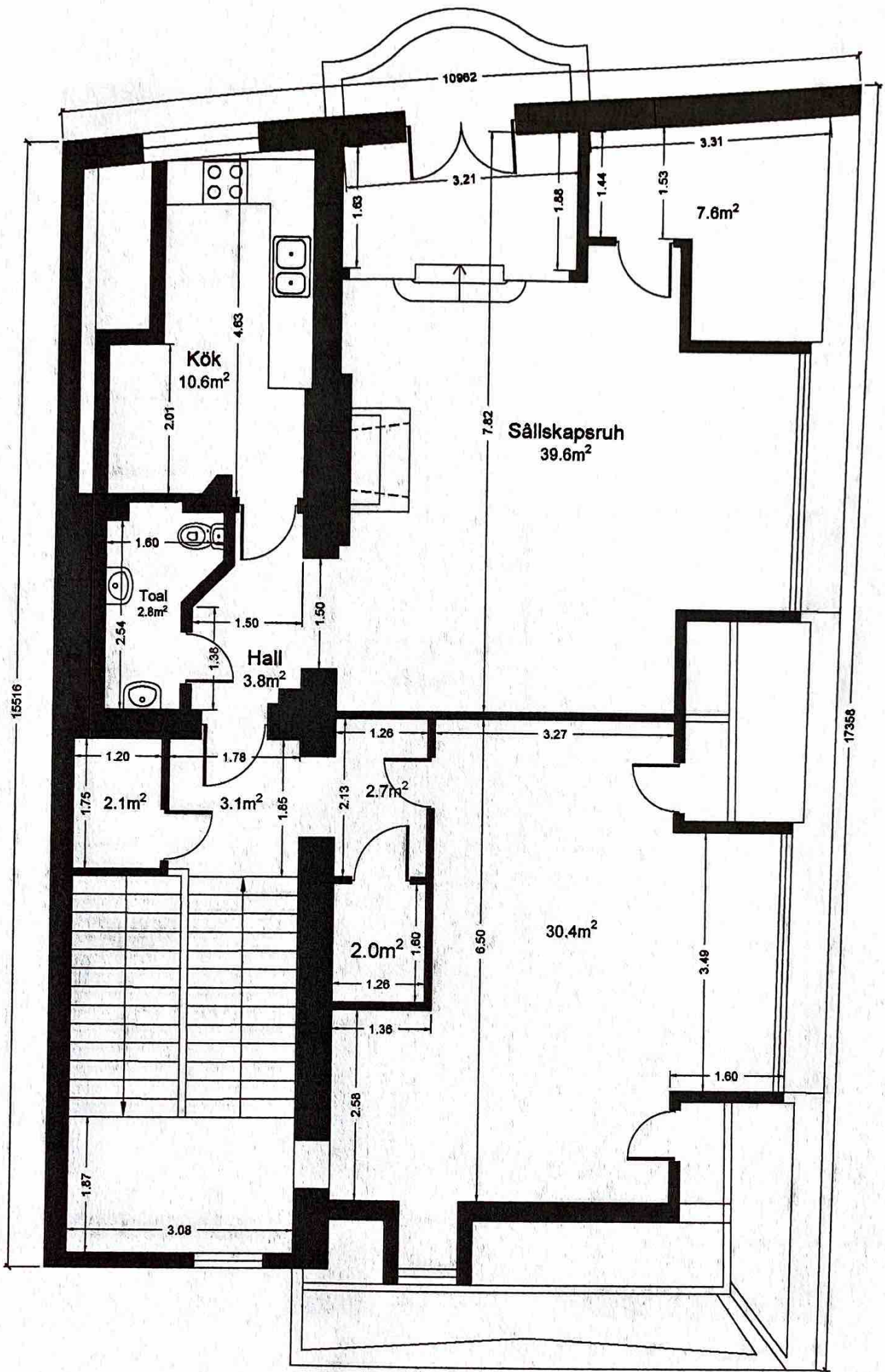
PLAN 5
