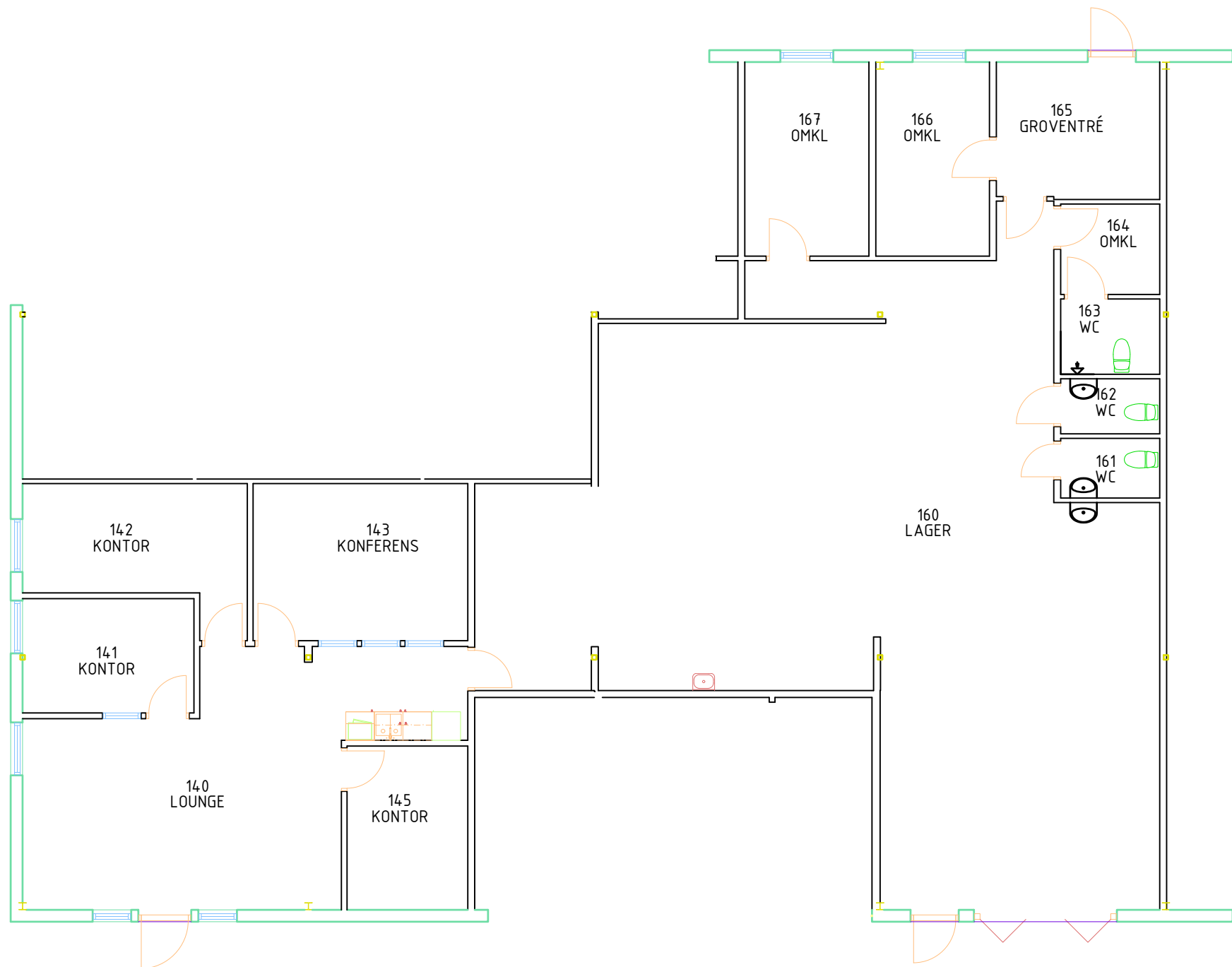
1-100 Plan 1
