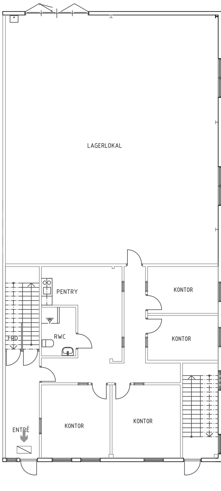
PLAN 1
