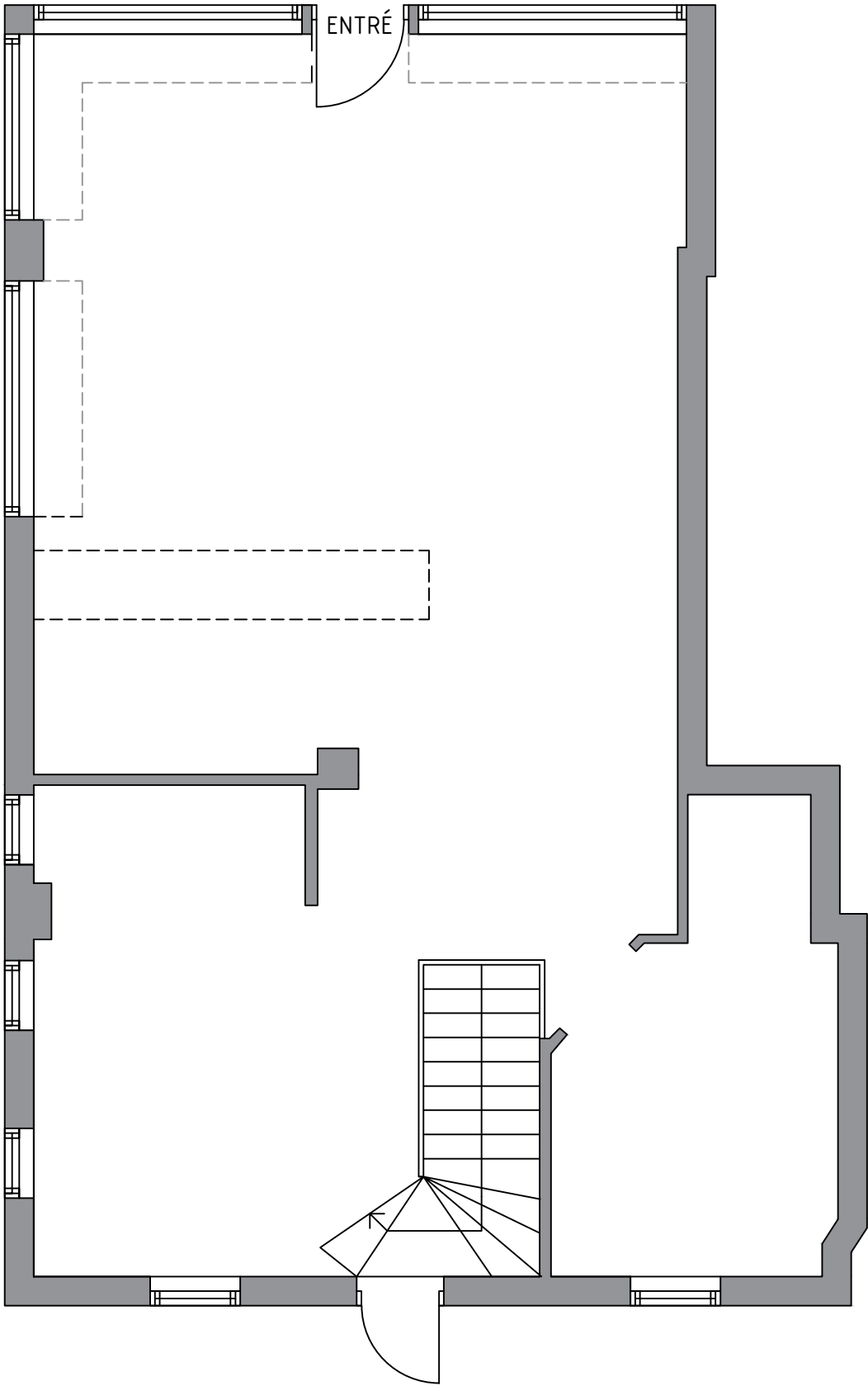
ENTRÉEPLAN LOA: 93,0 M 2
