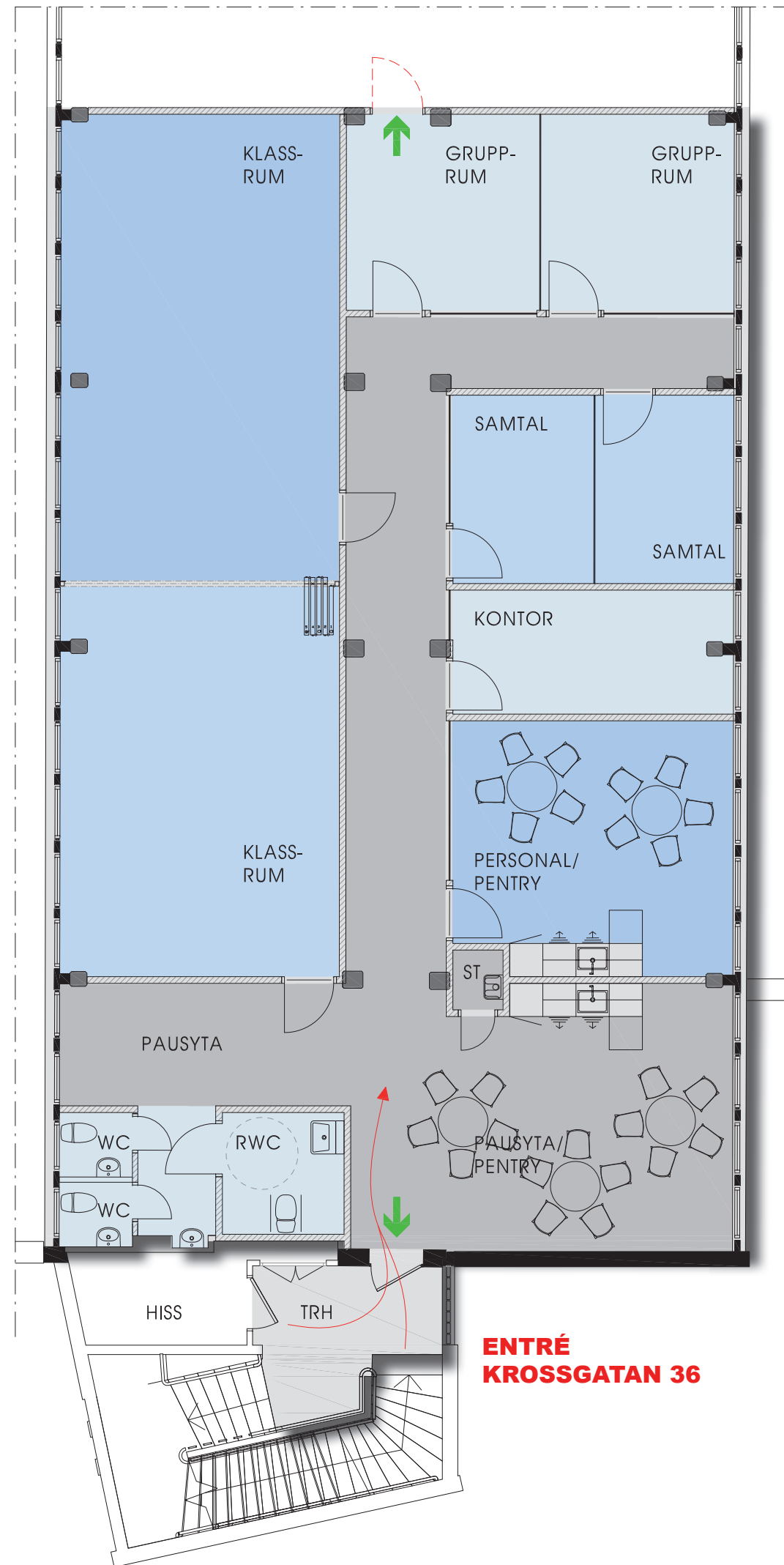
PLAN 5 A3 SKALA 1:100 LOA 250 KVM
