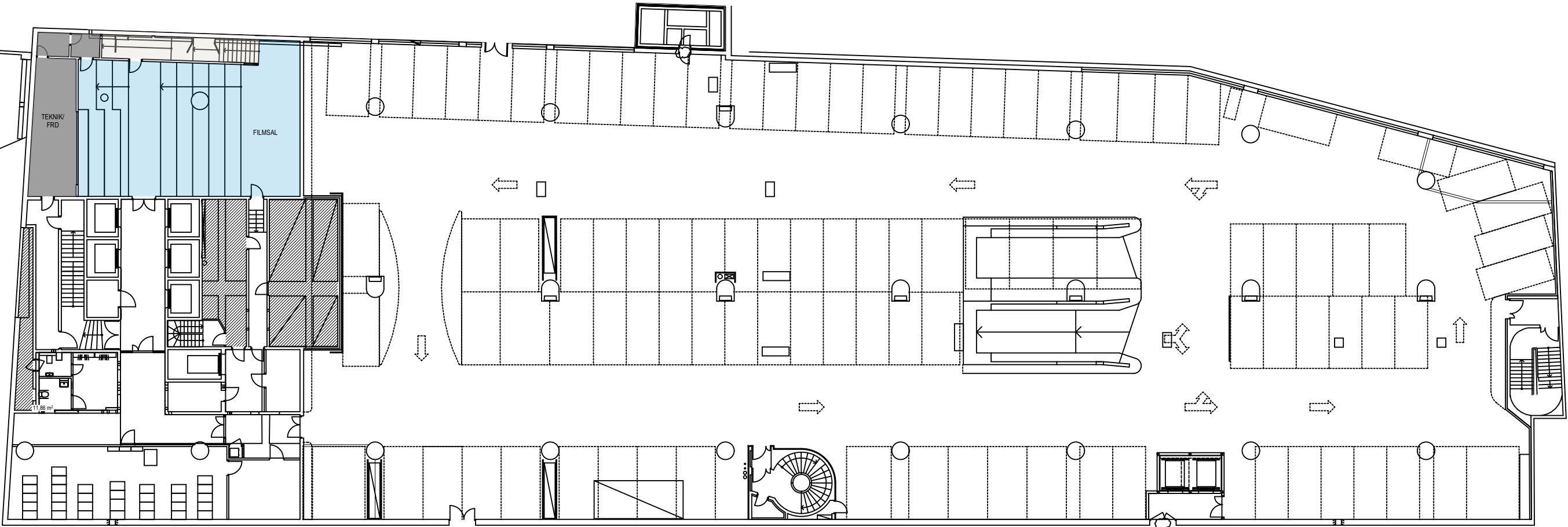
PLAN 1 1:300
