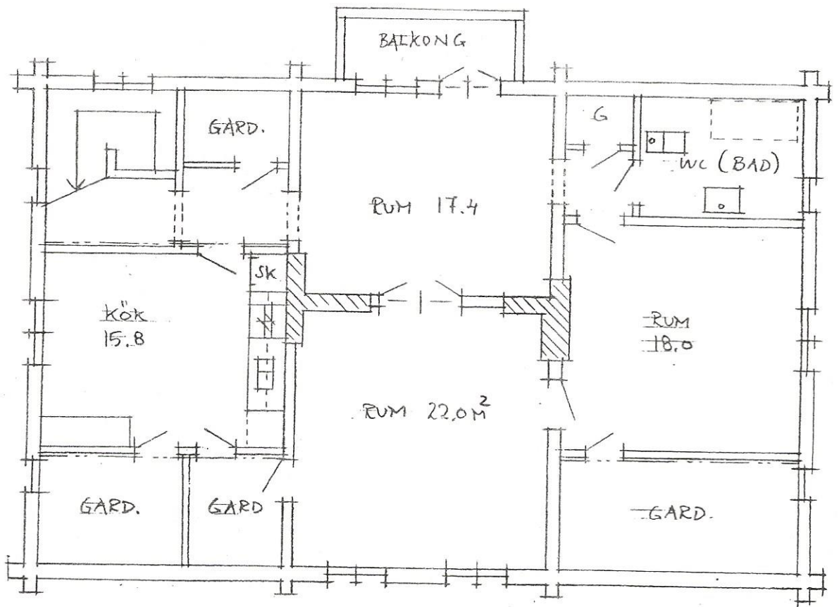
OVERPLAN
