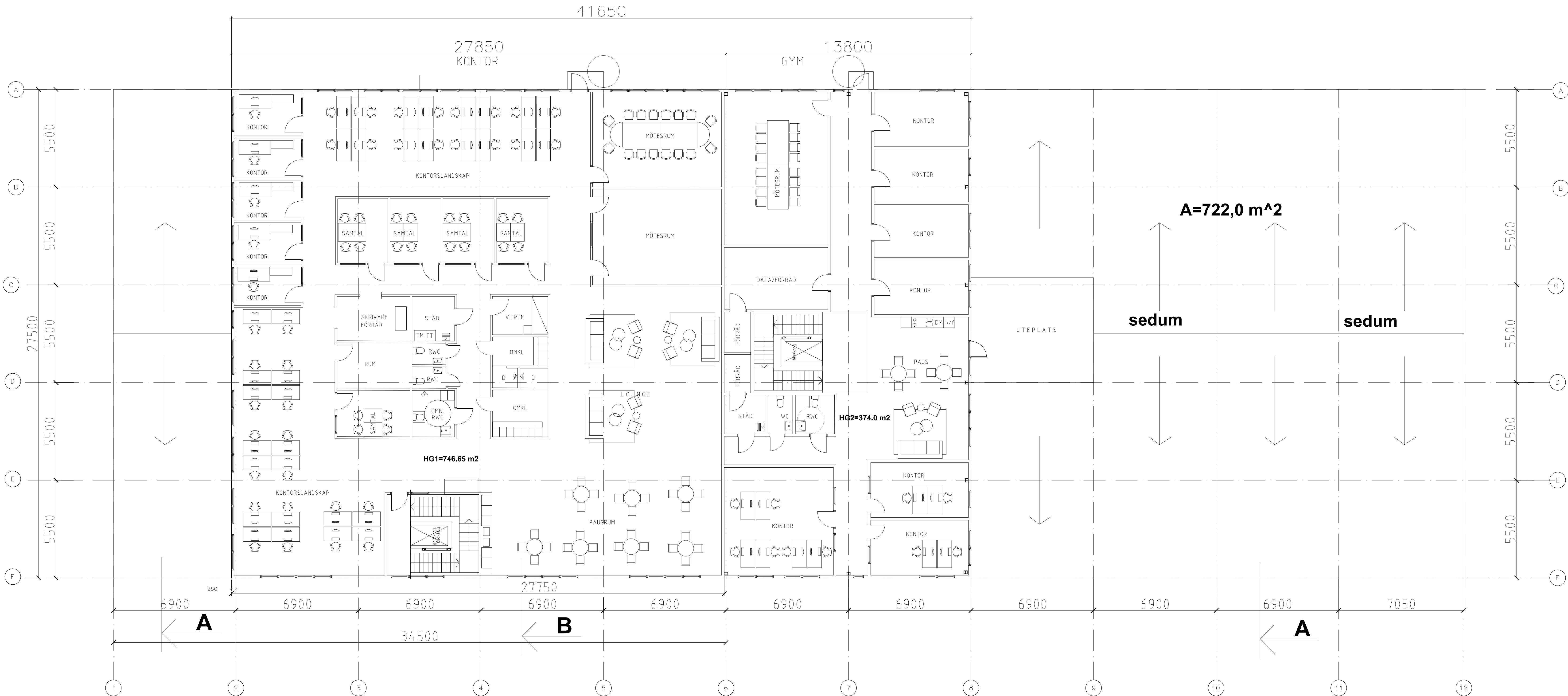
PLAN 1 BTA=1145,37 m^2
