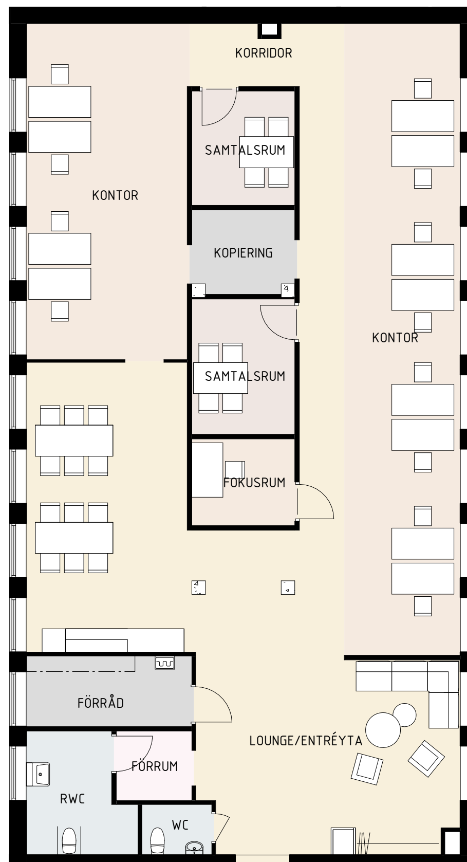
LOKAL 6 PLAN 2, skala 1:100 (A3) AREA 239 kvm
