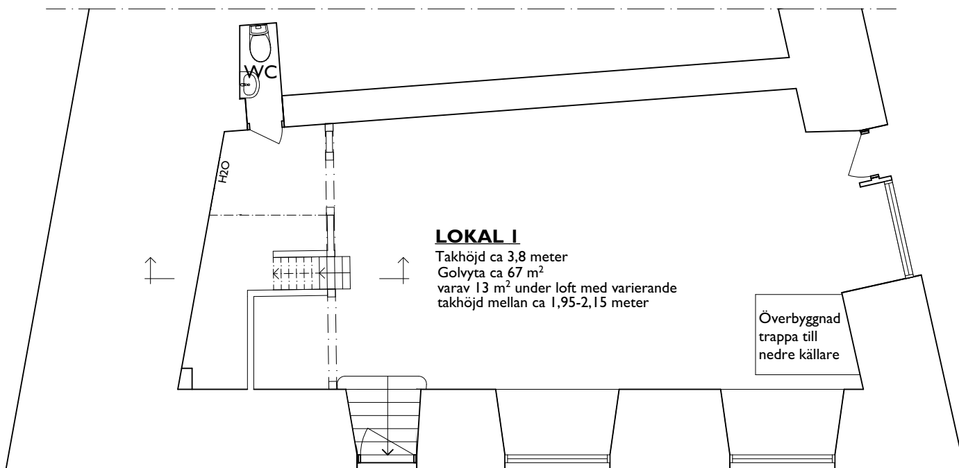
PLAN
