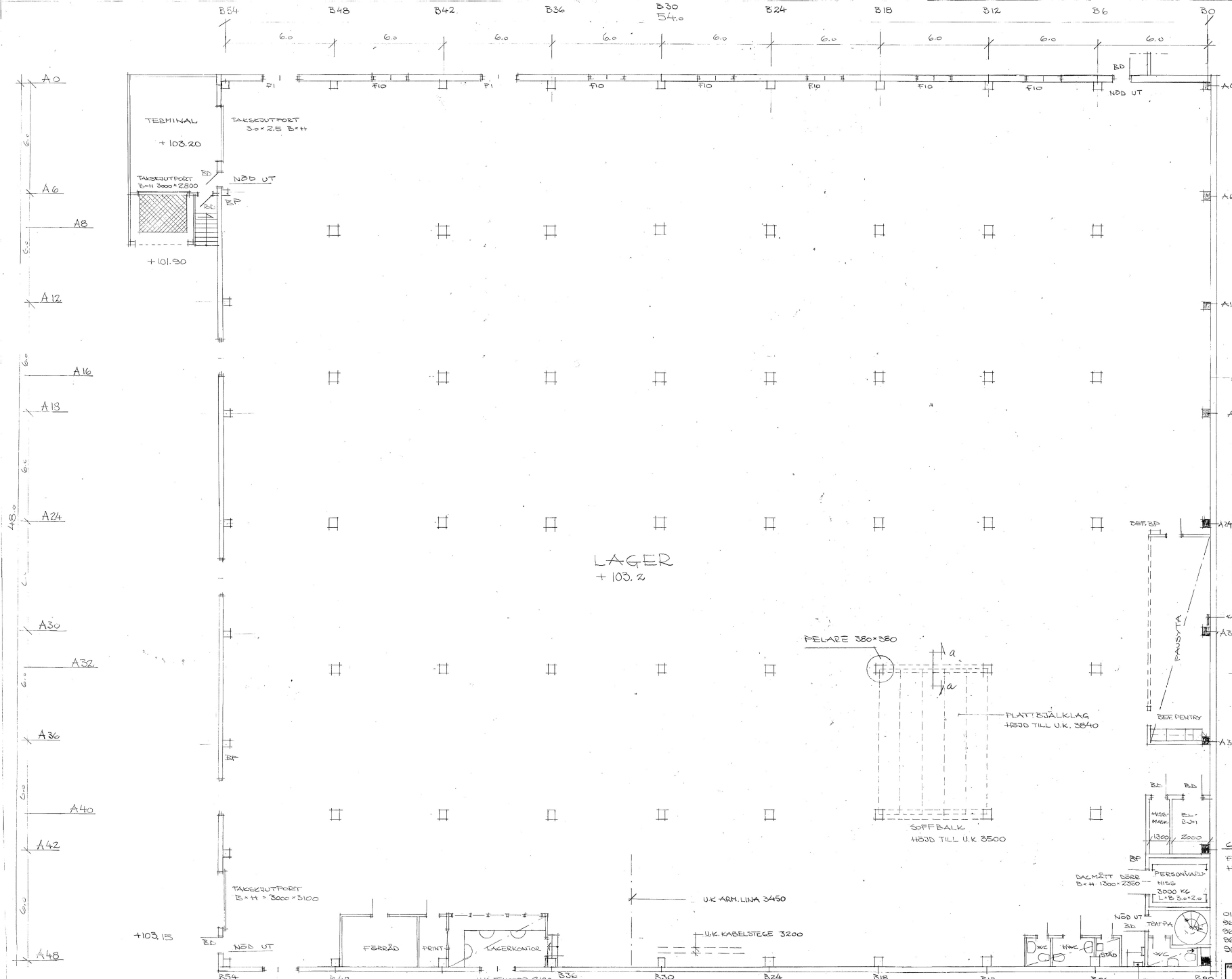
PLAN +103.2 1:100
