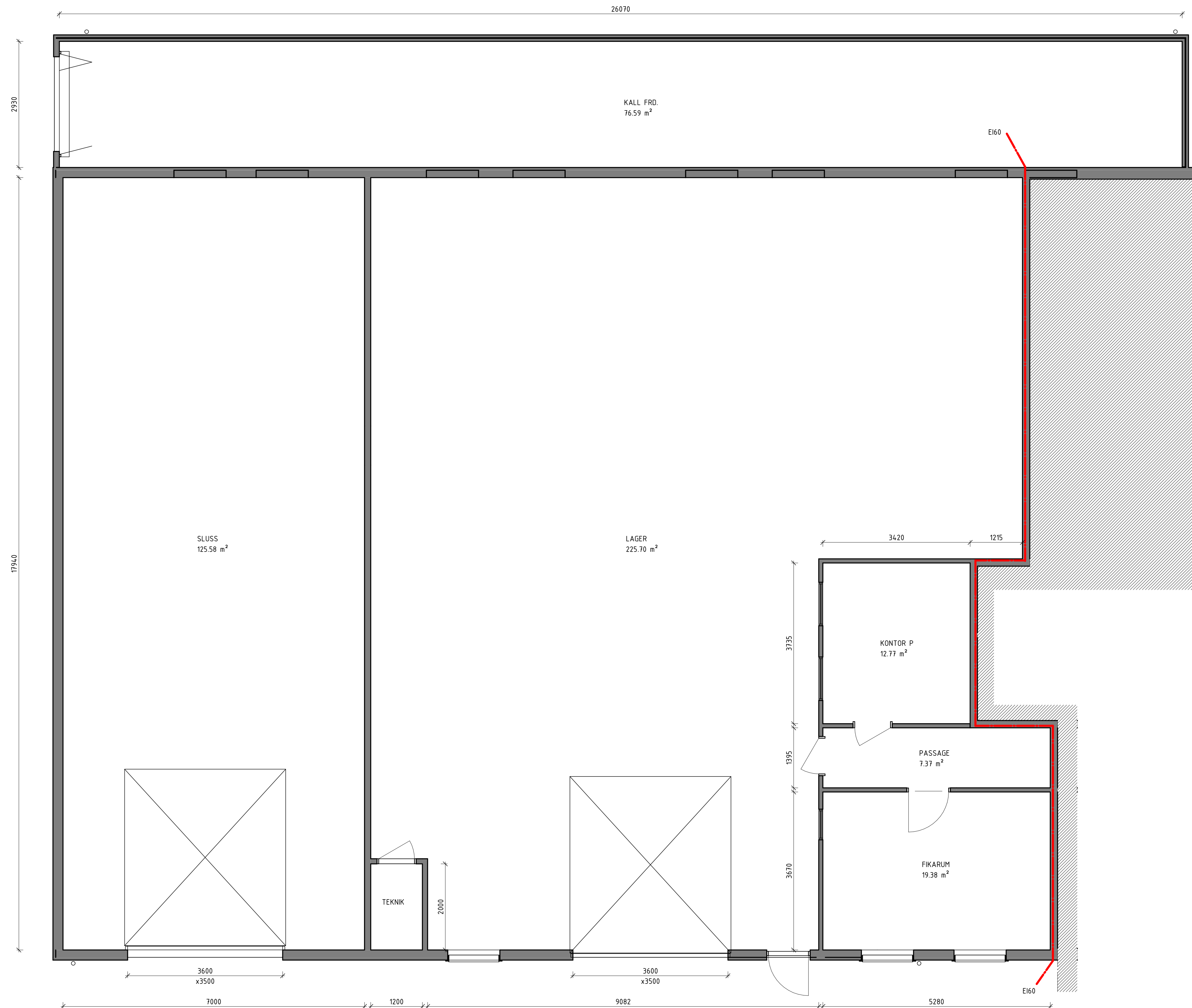
PLAN 1 - DELPLAN - SKISS 1 : 50 (A1)
