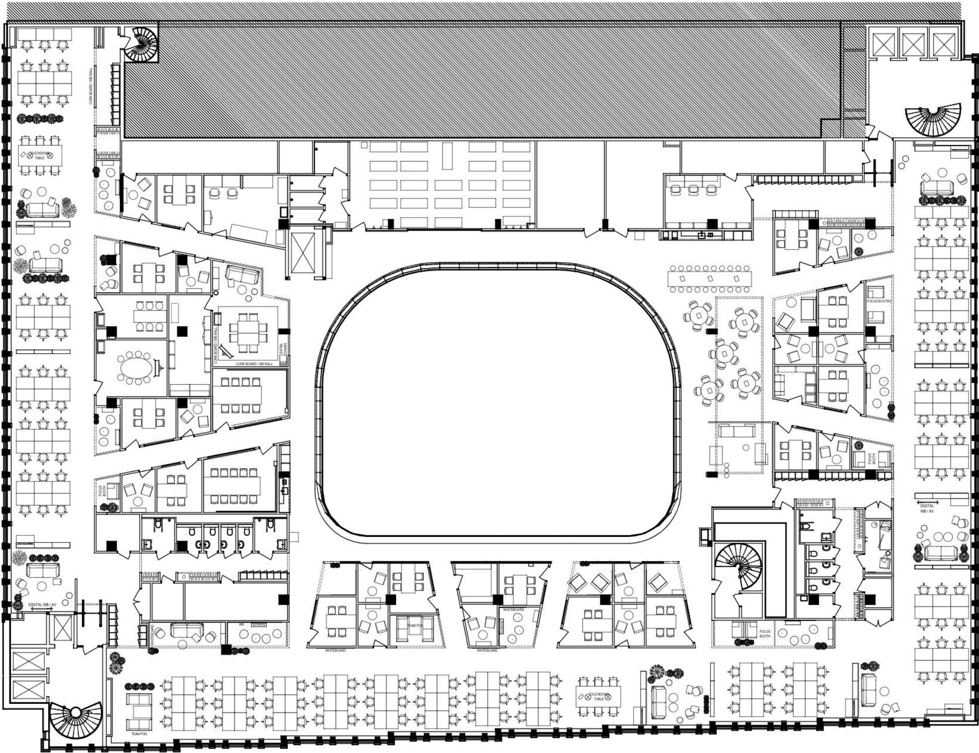
Floor 8
