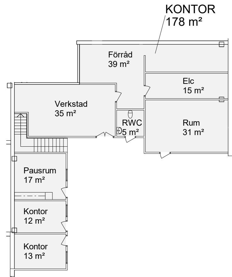
BOTTENPLAN
