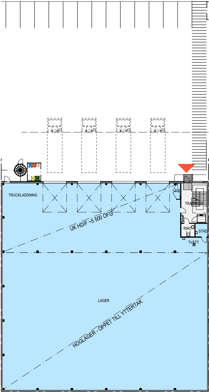
BOTTENPLAN
