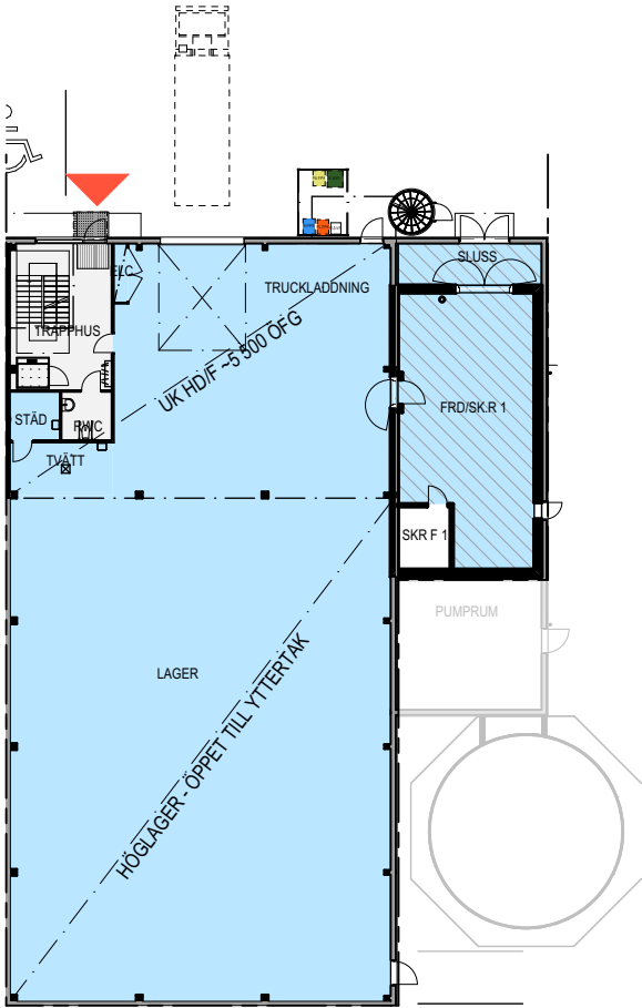
BOTTENPLAN
