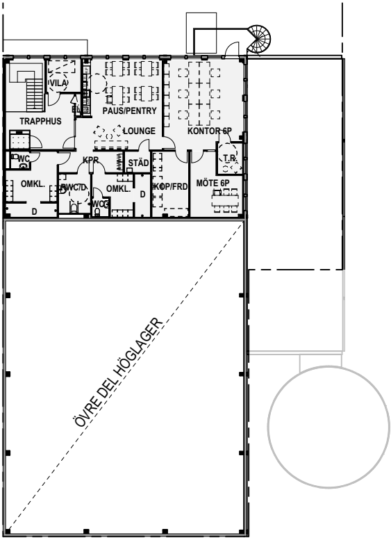
PLAN 1
