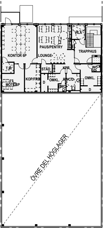
PLAN 1
