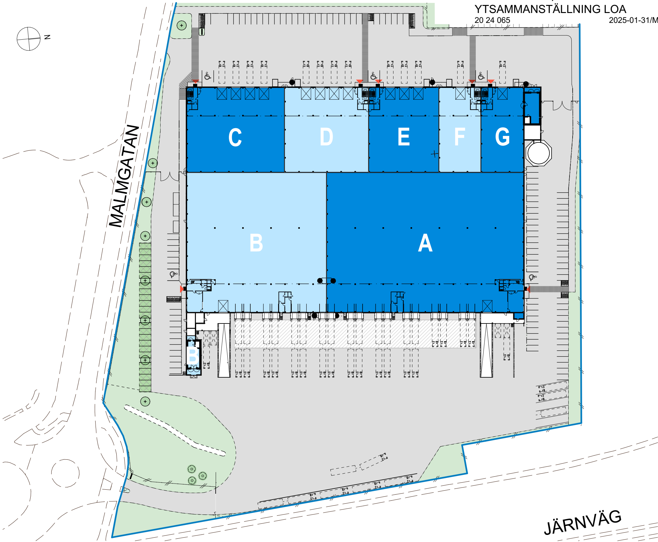
SITUATIONSPLAN
