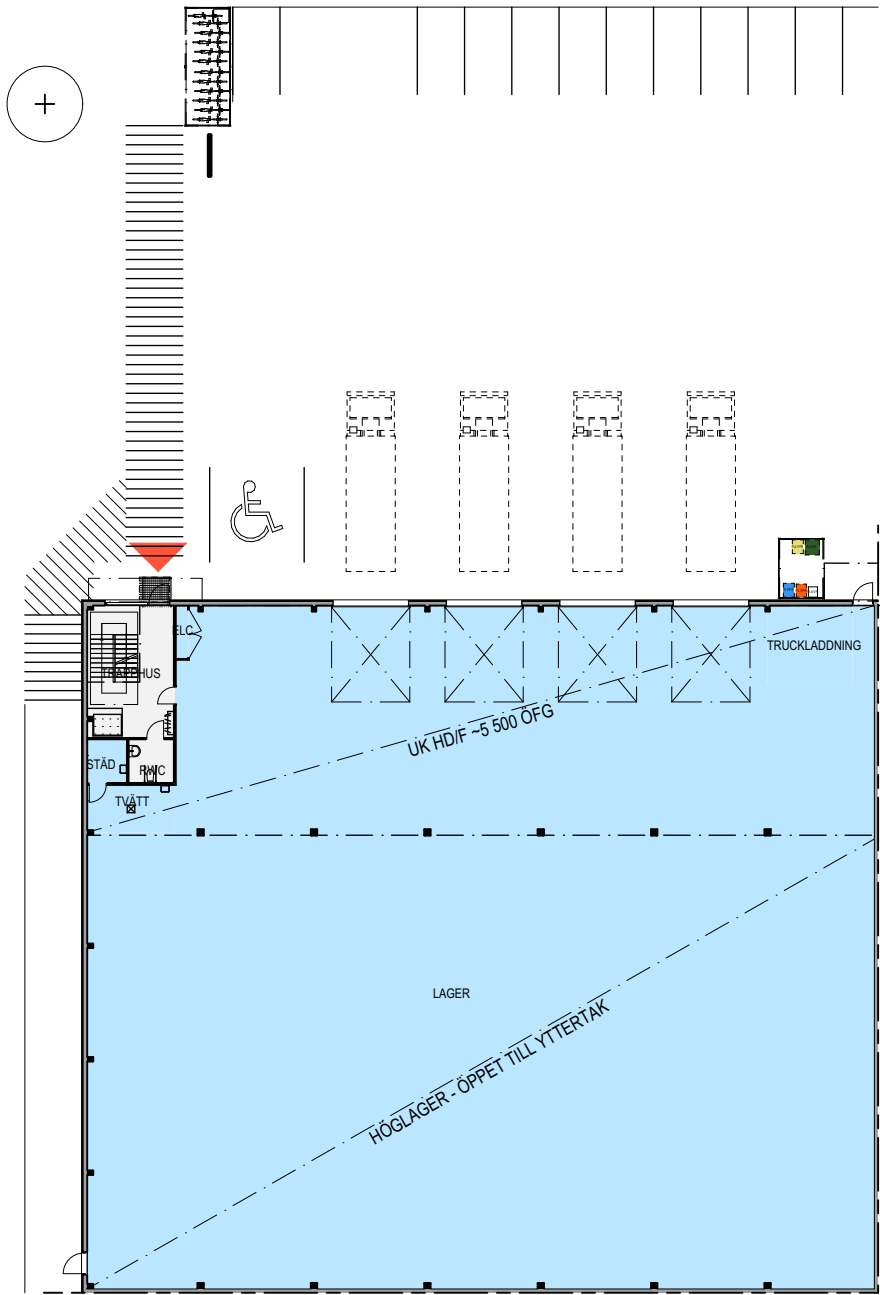
BOTTENPLAN
