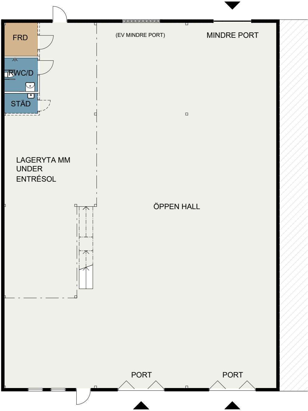
PLAN 1
