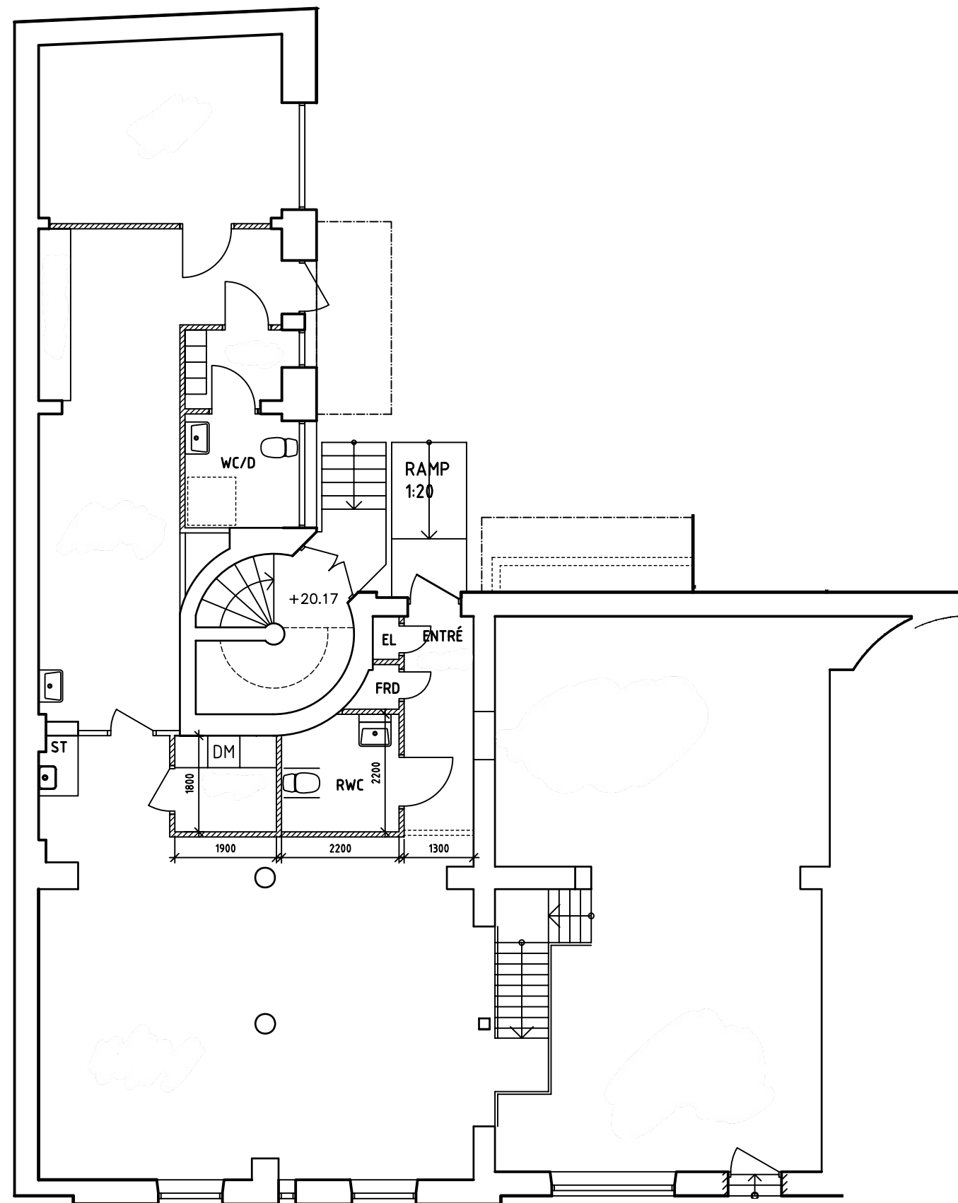
PLAN 2
