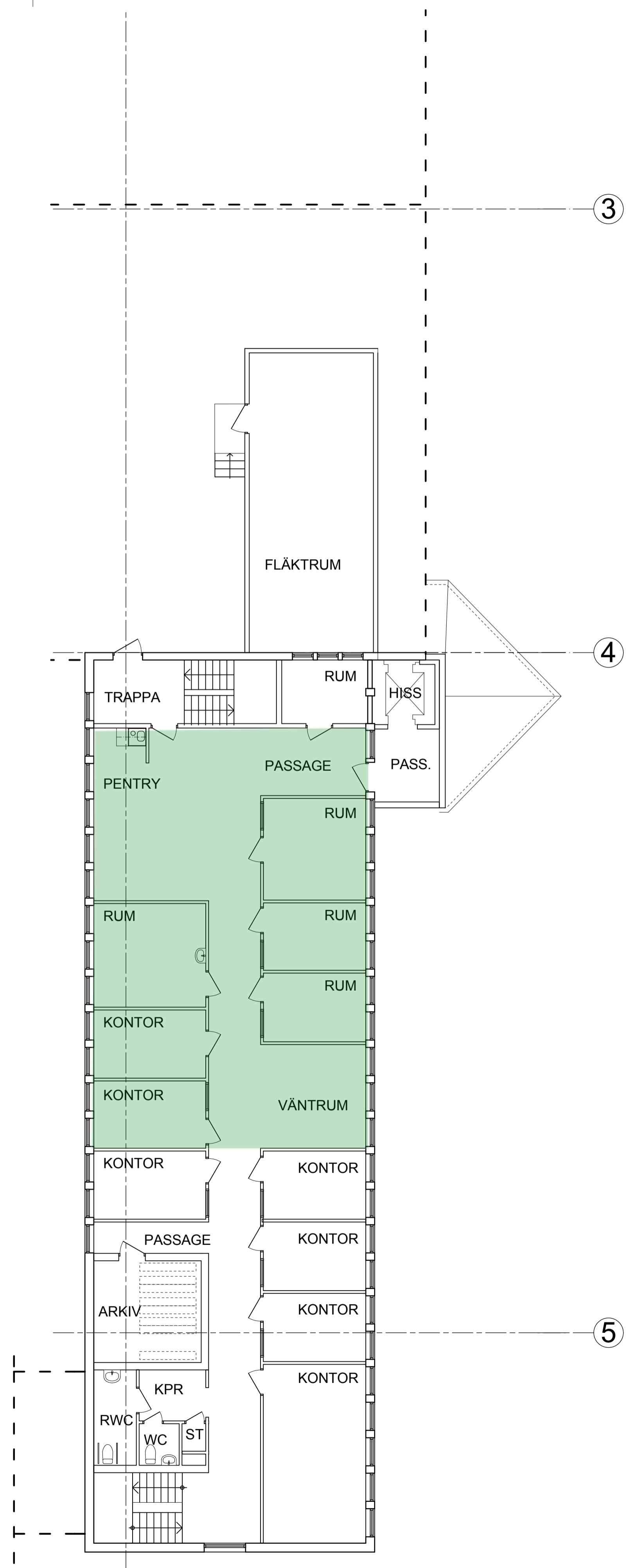
HUS 2, PLAN 4, 2 trappor
