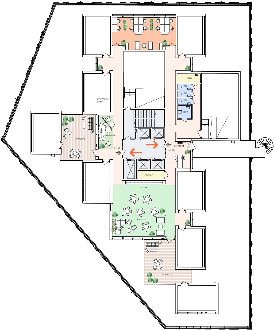
PLAN 15, 1:300
