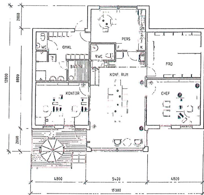
Plan 1
