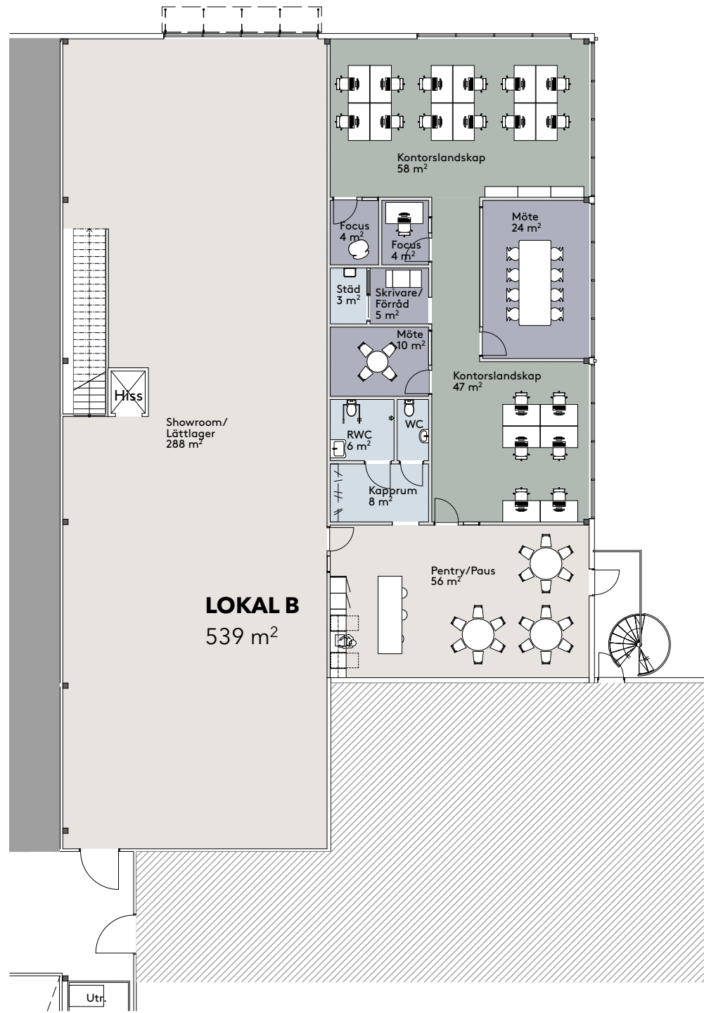
Plan 2 1:200
