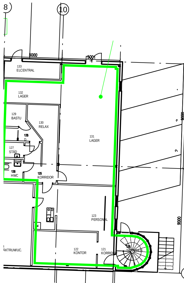
Bottenplan
