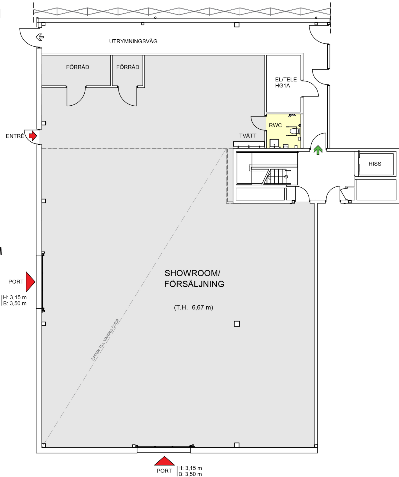
Markplan SHOWROOM
