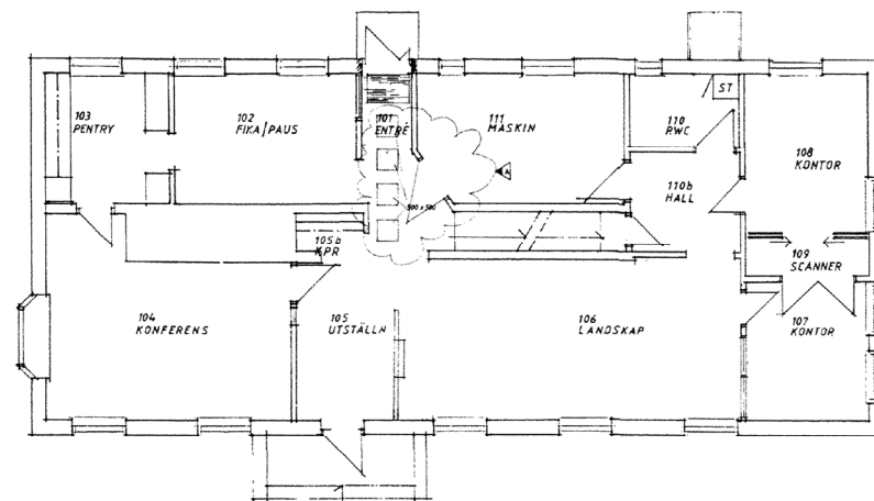
BOTTENPLAN
