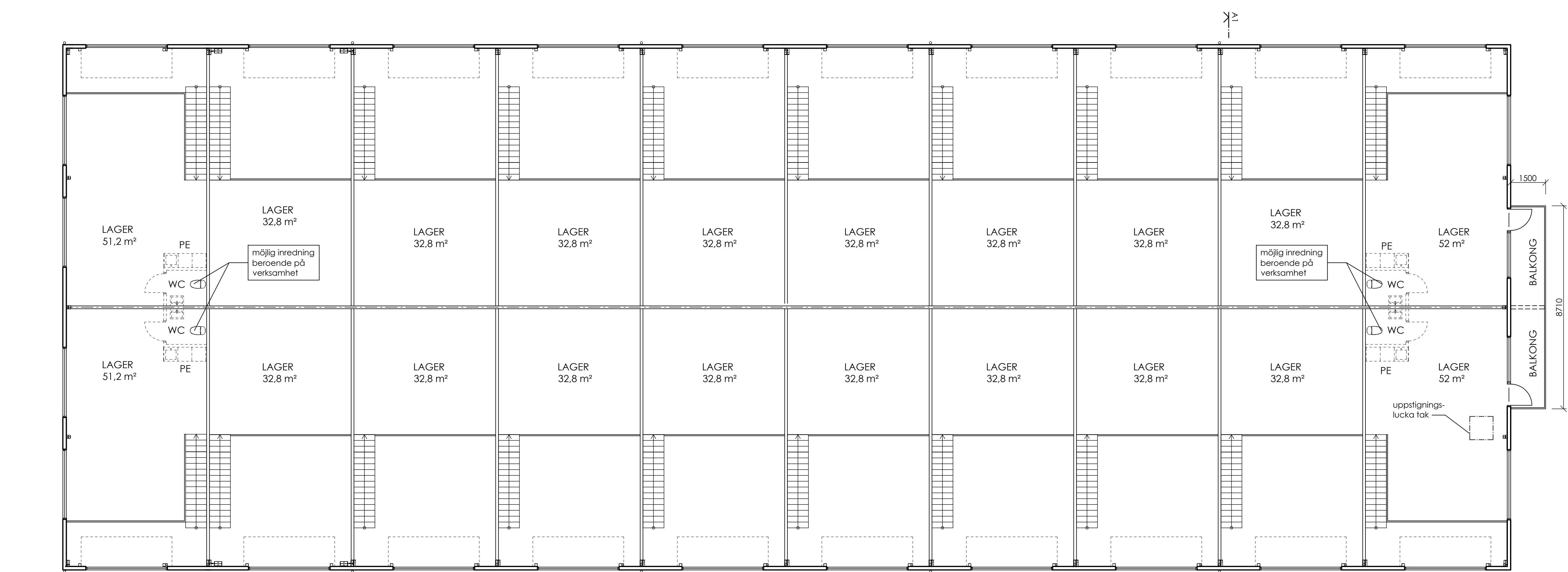
ENTRESOLPLAN SKALA 1:100 (A1)
