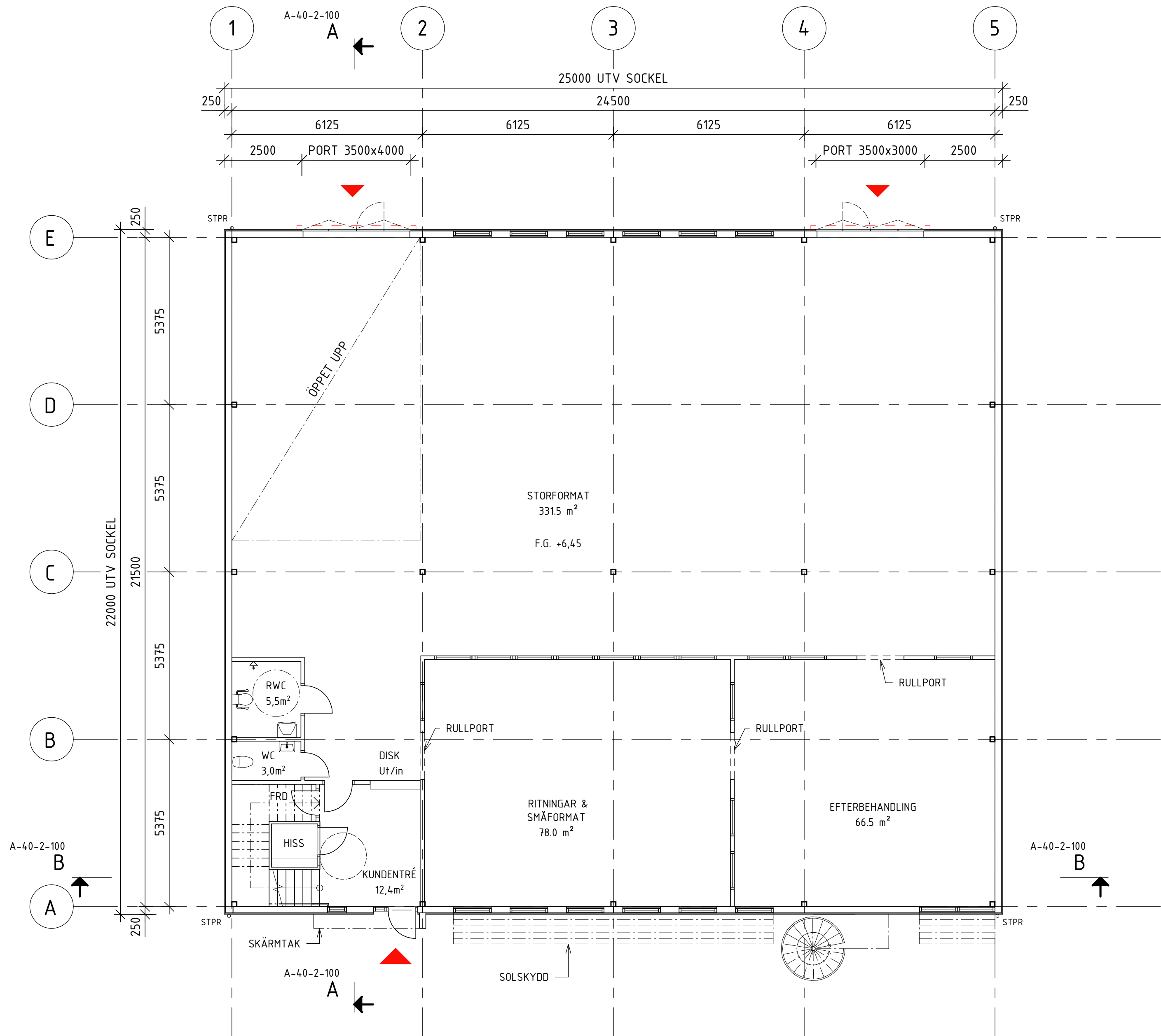
BOTTENPLAN
