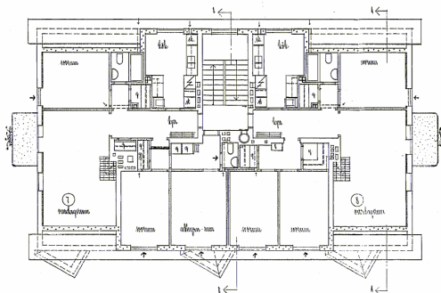
PLAN 2 TR
