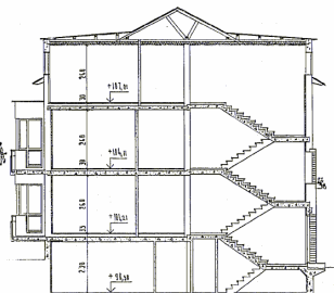
SECTION 3-3
