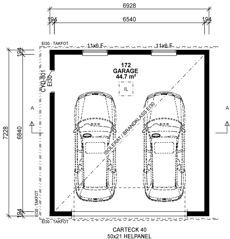
PLAN BYA = 50.1m²
