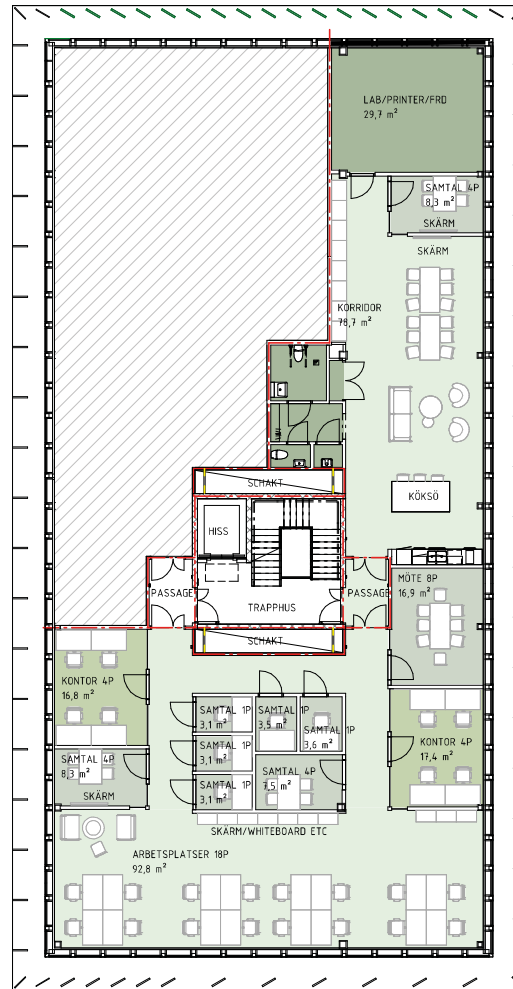
PLANRITNING, SKALA 1:200
