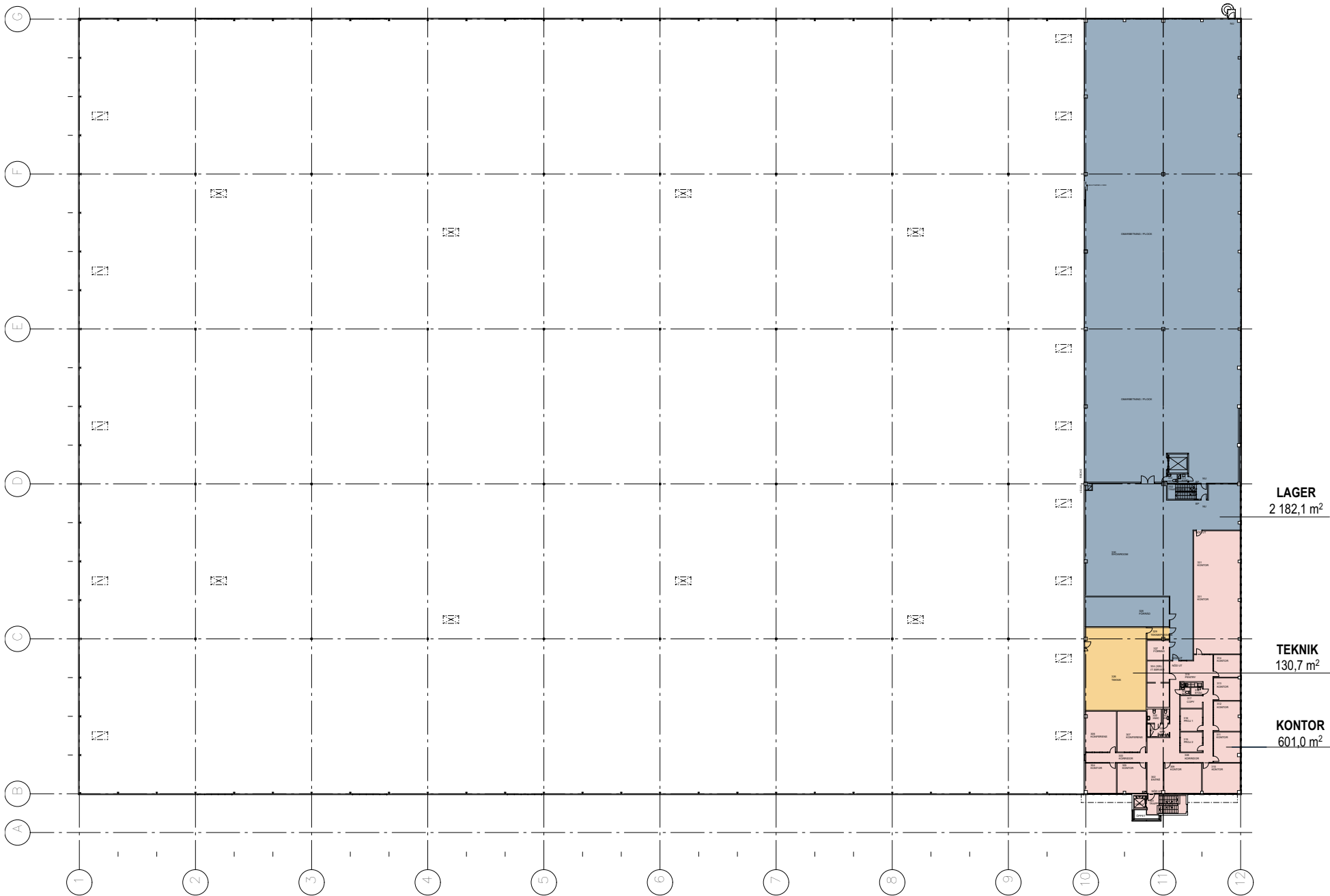
PLAN 3
