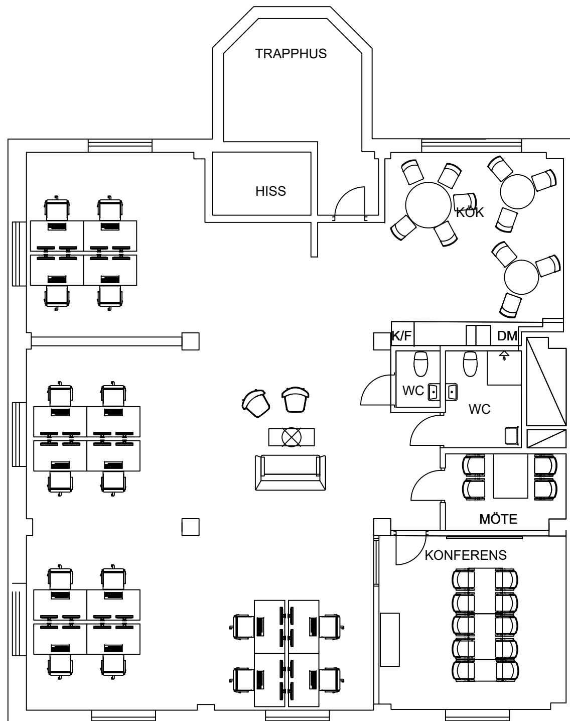
PLAN - 1 TR
